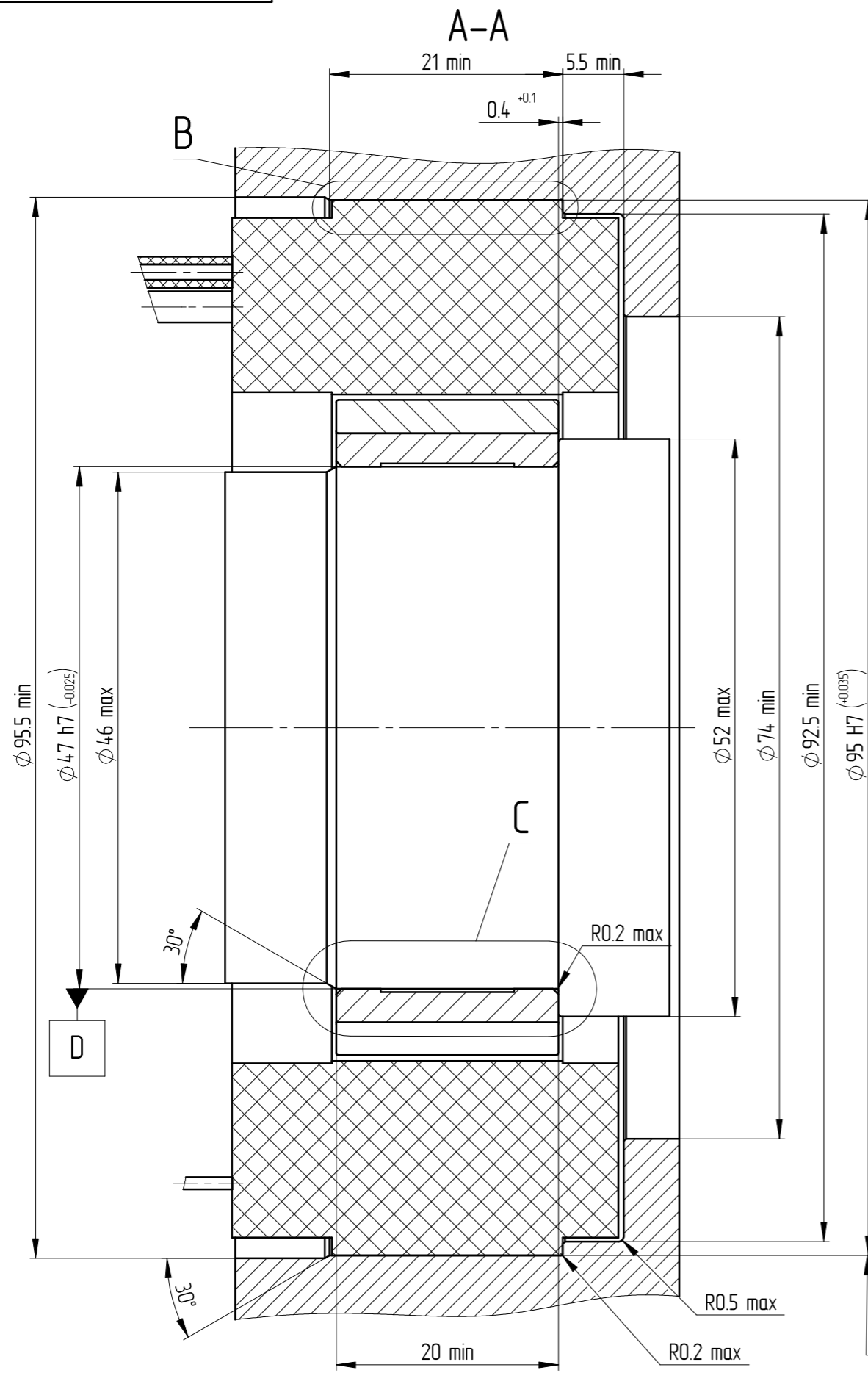
Fig. 2 The rotor-stator assembly in a housing
